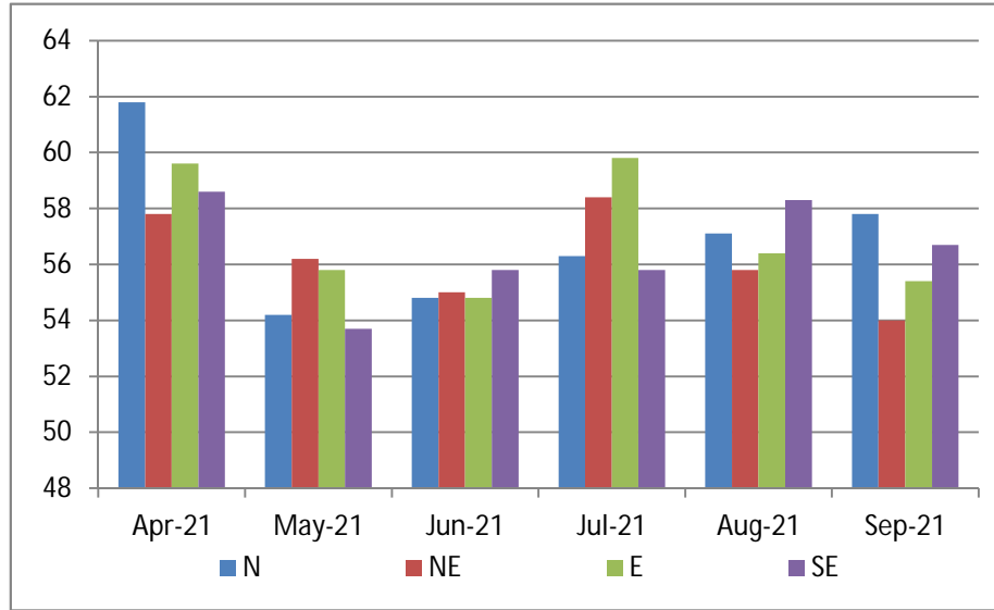
PM10
